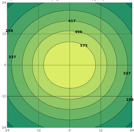
Equinox 1000 PPFD Map @ 24" Above Canopy (Open 4'x4' Area)
